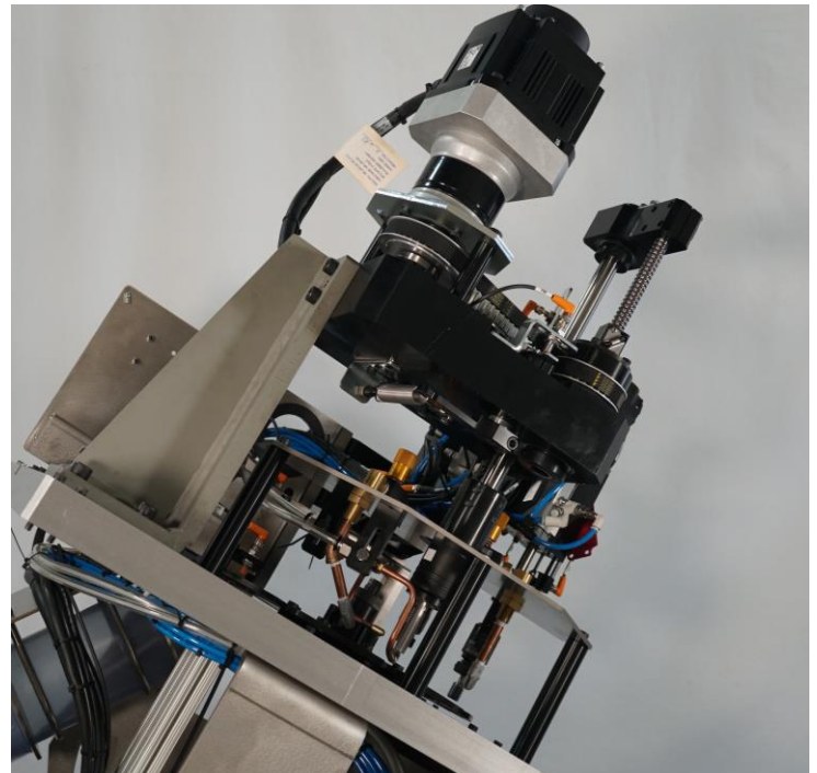
An AR Tapper for a high volume slidedown line.
